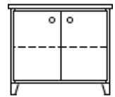
2 Door Base Cabinet w/1 adjustable shelf 36W x 20D x 30H
